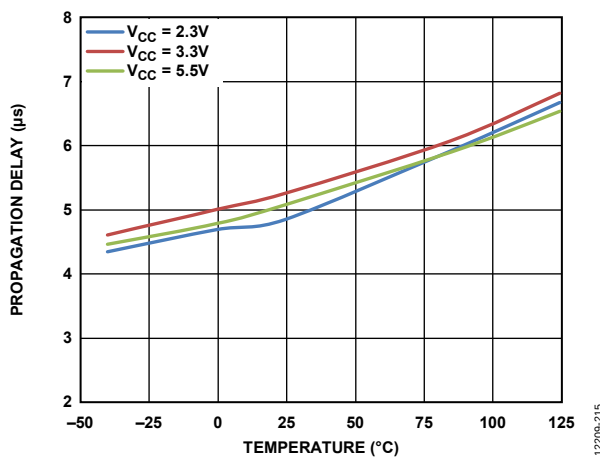
Figure 15. Propagation Delay vs. Temperature, Low to High, V_{OD} = 10mV
