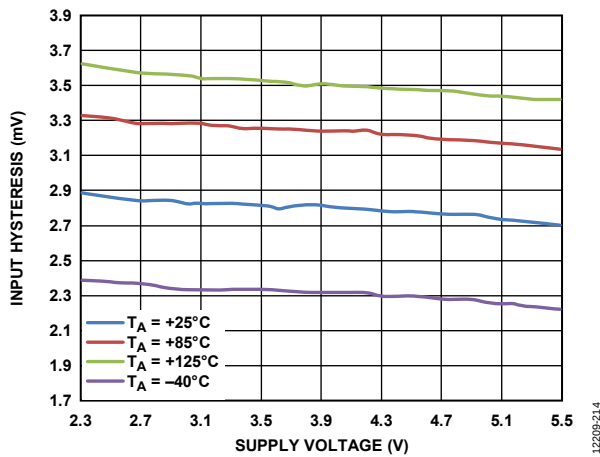
Figure 14. Input Hysteresis vs. Supply Voltage ( V_{CC} ), V_{CM} = 1V for Various Temperatures
