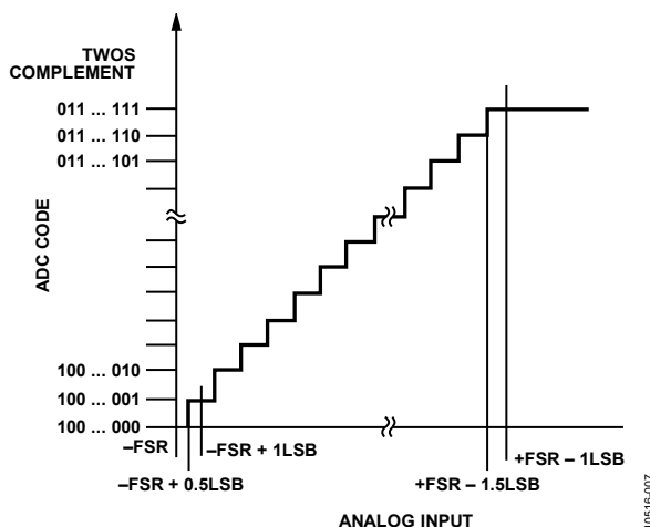
Figure 54. ADC Ideal Transfer Function
