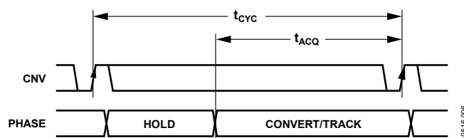
Figure 53. ADAS3022 System Timing
