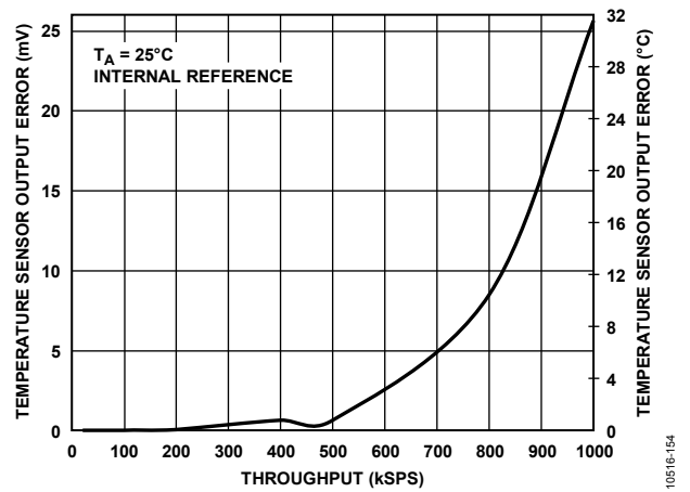
Figure 51. Temperature Sensor Output Error vs. Throughput
