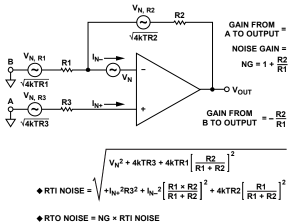
Figure 57. Operational Amplifier Noise Analysis Model
