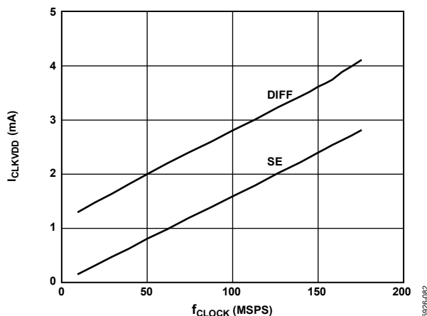
Figure 84. I_{CLKVDD} vs. f_{CLOCK} at CLKVDD = 3.3\text{ V}
