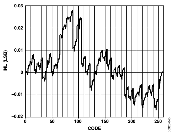
Figure 45. AD9704 Typical Uncalibrated INL
