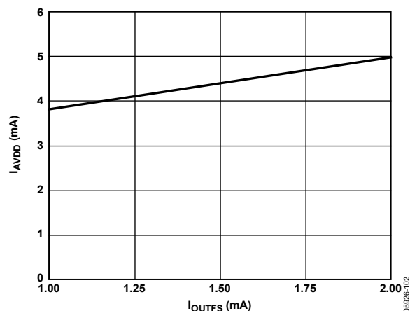
Figure 81. I_{AVDD} vs. I_{OUTFS} at AVDD = 1.8\text{ V}
