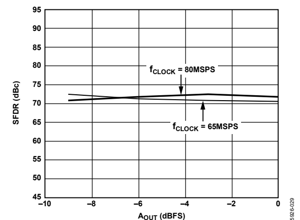
Figure 32. SFDR vs. A_{OUT} at f_{OUT} = f_{CLOCK}/5
