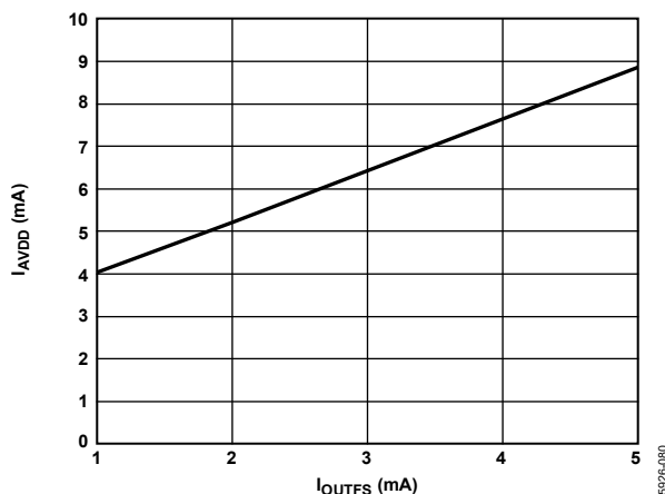
Figure 80. I_{AVDD} vs. I_{OUTFS} at AVDD = 3.3\text{ V}
