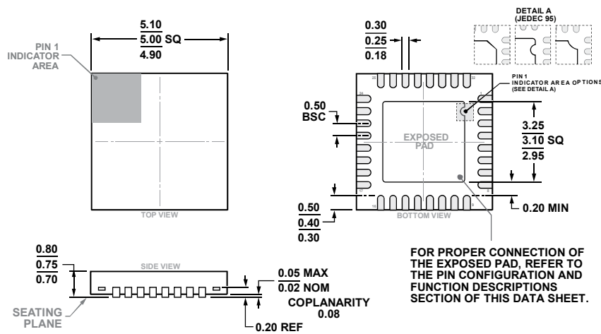
Figure 91. 32-Lead Lead Frame Chip Scale Package [LFCS] 5 mm x 5 mm and 0.75 mm Package Height (CP-32-7) Dimensions shown in millimeters
