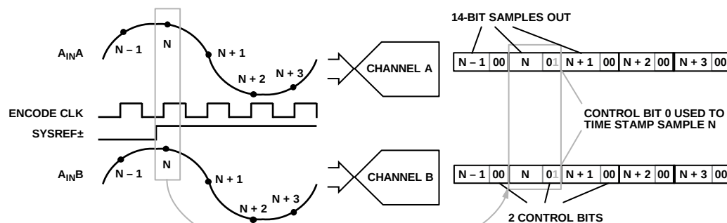
Figure 97. Timestamping—CS = 2 (Register 0x058F, Bits[7:6] = 2 Decimal), Control Bit 0 is SYSREF± (Register 0x0559, Bits[2:0] = 5 Decimal)
