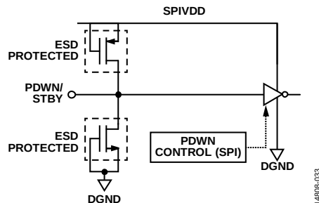
Figure 53. PDWN/STBY Input
