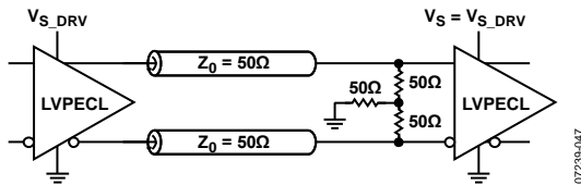
Figure 60. DC-Coupled 3.3 V LVPECL Y-Termination
