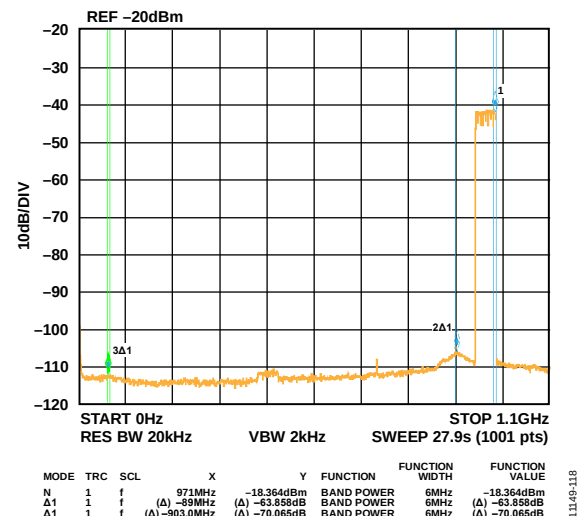
Figure 107. Eight Carrier at 950 MHz Output
