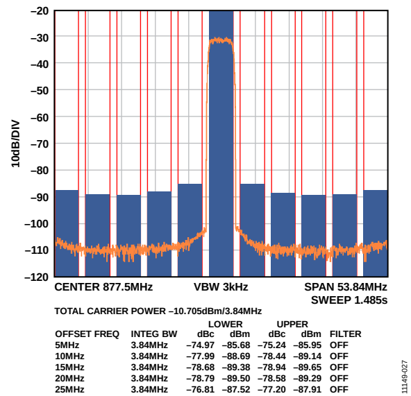
Figure 21. Single-Carrier W-CDMA at 877.5 MHz
