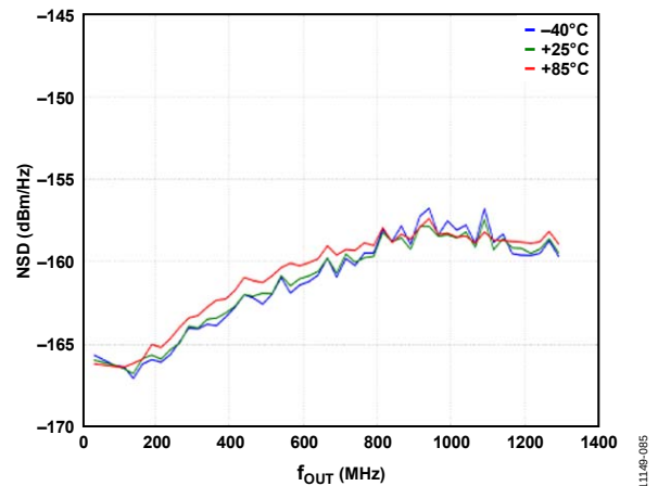
Figure 78. Single-Tone NSD vs. f_{OUT} over Temperature
