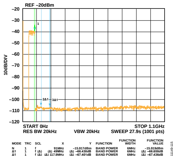
Figure 104. Eight Carrier at 70 MHz Output
