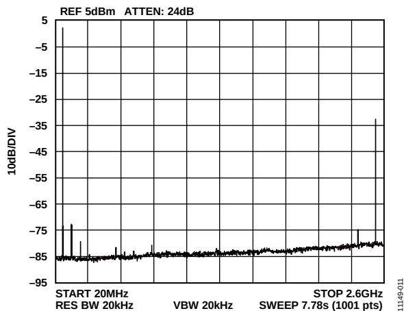
Figure 10. Single-Tone Spectrum at f_{OUT} = 70 \text{ MHz}
