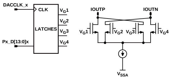
Figure 143. Quad-Switch Architecture
