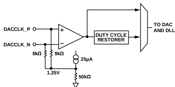
Figure 147. Clock Input
