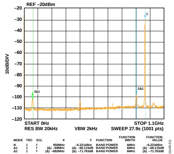
Figure 105. Single Carrier at 950 MHz Output
