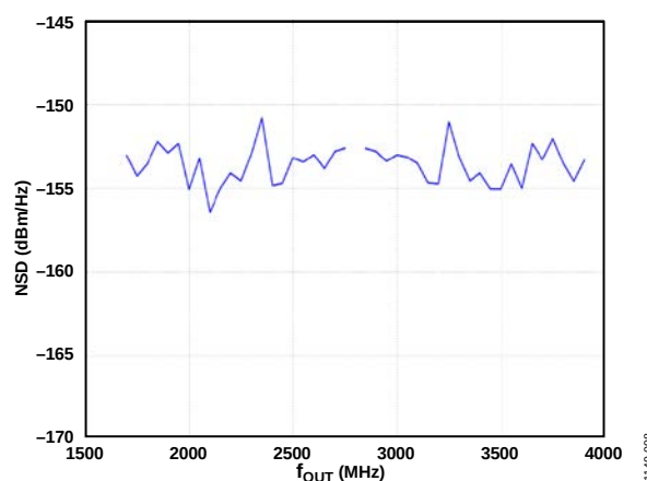
Figure 89. W-CDMA NSD vs. f_{OUT}
