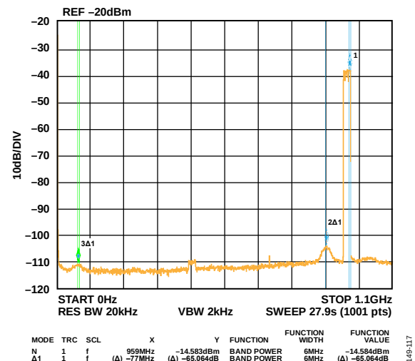
Figure 106. Four Carrier at 950 MHz Output
