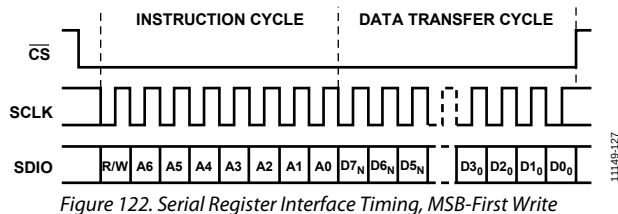
Figure 122. Serial Register Interface Timing, MSB-First Write
