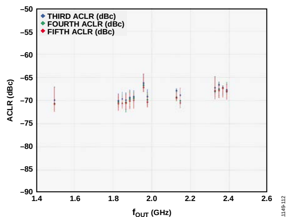
Figure 101. Four-Carrier W-CDMA ACLR vs. f_{OUT} (Third ACLR, Fourth ACLR, Fifth ACLR)
