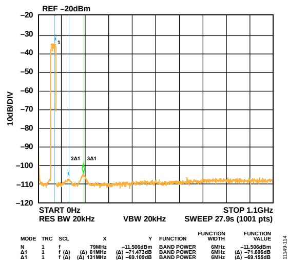
Figure 103. Four Carrier at 70 MHz Output
