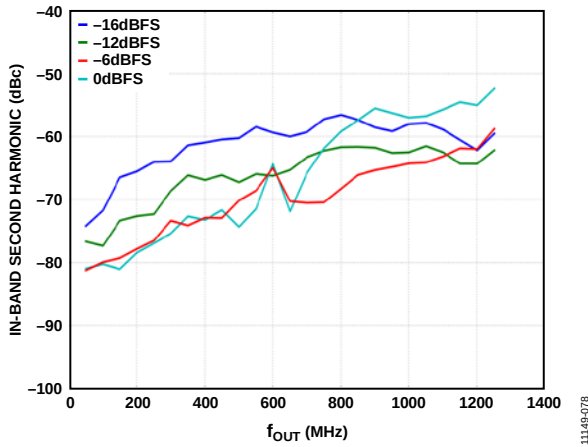
Figure 69. SFDR for Second Harmonic vs. f_{OUT} over Digital Full Scale
