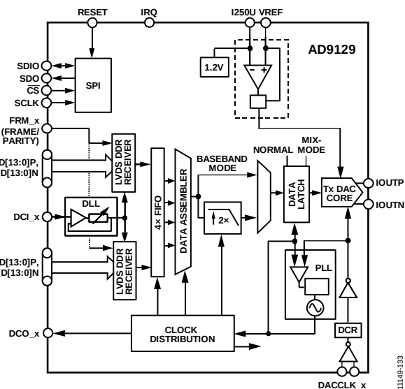
Figure 128. Functional Block Diagram of the AD9119/AD9129
