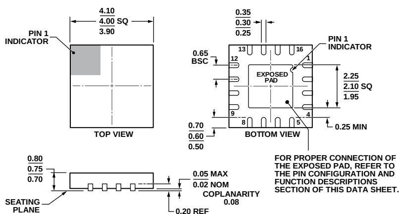
Figure 22. 16-Lead Lead Frame Chip Scale Package [LFCSP_WQ] 4 mm × 4 mm Body, Very Very Thin Quad (CP-16-23) Dimensions shown in millimeters
