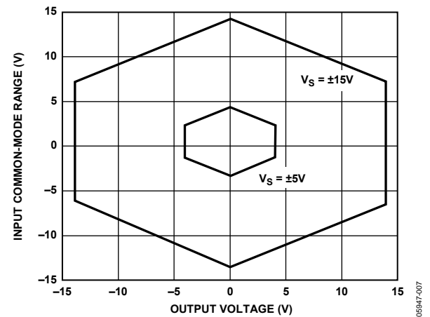
Figure 8. Input Common-Mode Range vs. Output Voltage, G = 1
