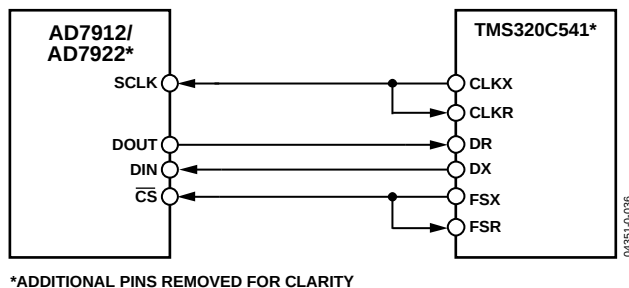
Figure 39. Interfacing to the TMS320C541
