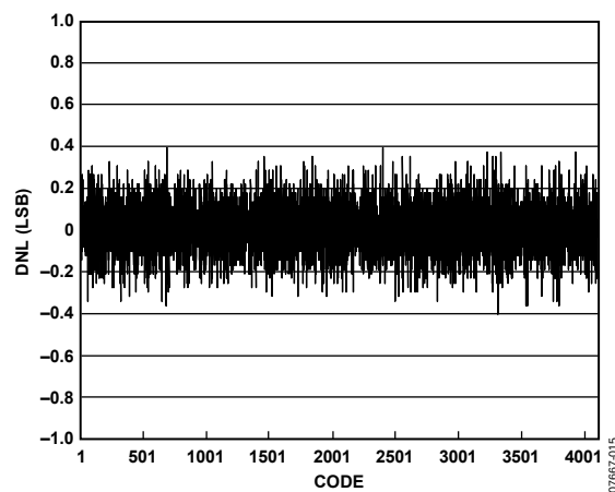
Figure 15. ADC DNL
