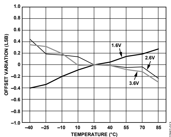
Figure 13. ADC Offset Variation vs. Temperature
