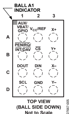
Figure 5. AD7879/AD7889 WLCSP Pin Configuration
