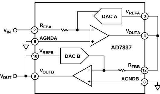
Figure 17. Dual PGA Circuit
