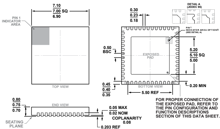
COMPLIANT TO JEDEC STANDARDS MO-220-WKCD-4 Figure 48. 48-Lead Lead Frame Chip Scale Package [LFCSP] 7 mm x 7 mm Body and 0.75 mm Package Height (CP-48-4)
