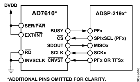
Figure 46. Interfacing the AD7610 to SPI Interface
