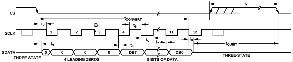
Figure 31. AD7468 Serial Interface Timing Diagram
