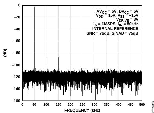
Figure 5. AD7367 FFT
