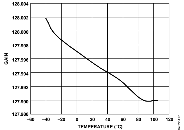
Figure 17. Gain Error (Gain = 128)
