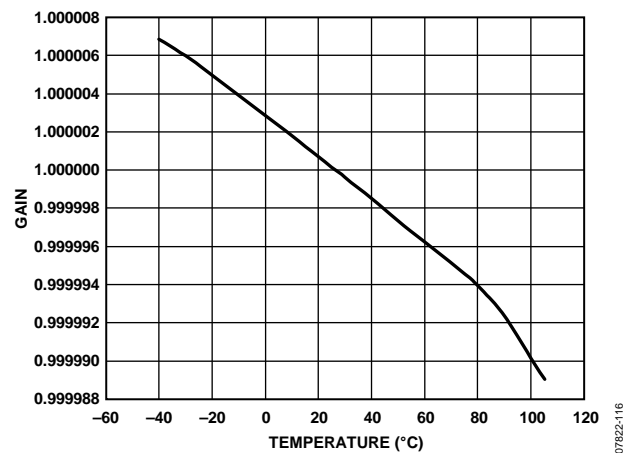
Figure 16. Gain Error (Gain = 1)
