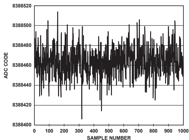
Figure 7. Noise (Analog Input Buffers Disabled, V_{REF} = 5\text{ V} , Output Data Rate = 250 kSPS)
