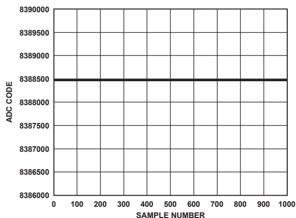
Figure 5. Noise (Analog Input Buffers Disabled, V_{REF} = 5\text{ V} , Output Data Rate = 5 SPS)
