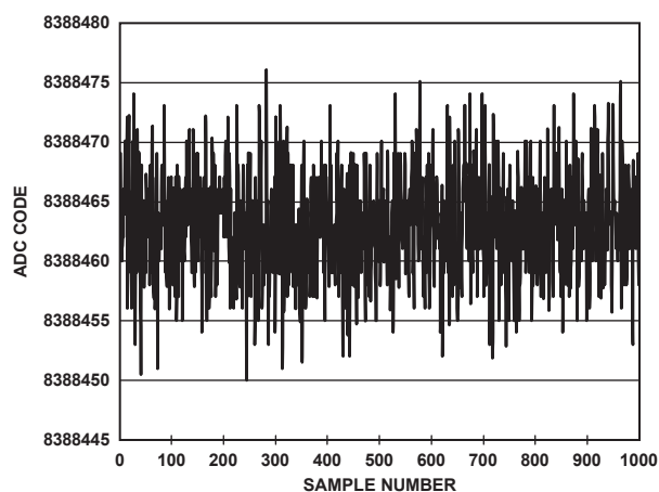
Figure 6. Noise (Analog Input Buffers Disabled, V_{REF} = 5\text{ V} , Output Data Rate = 10 kSPS)
