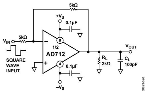
Figure 26. Unity-Gain Inverter
