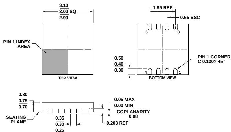
COMPLIANT TO JEDEC STANDARDS MO-229-WEEC-2 Figure 56. 8-Lead Lead Frame Chip Scale Package [LF CSP_WD] 3 mm × 3 mm Body, Very Very Thin, Dual Lead (CP-8-15) Dimensions shown in millimeters
