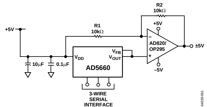
Figure 51. Bipolar Operation with the AD5660
