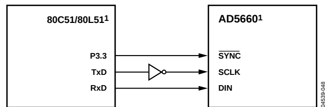
Figure 48. AD5660-to-80C51/80L51 Interface
