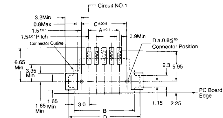
PC Board Layout (Component Side) (Applicable board thickness=0.8mm Min.)
