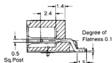
Section X-X
