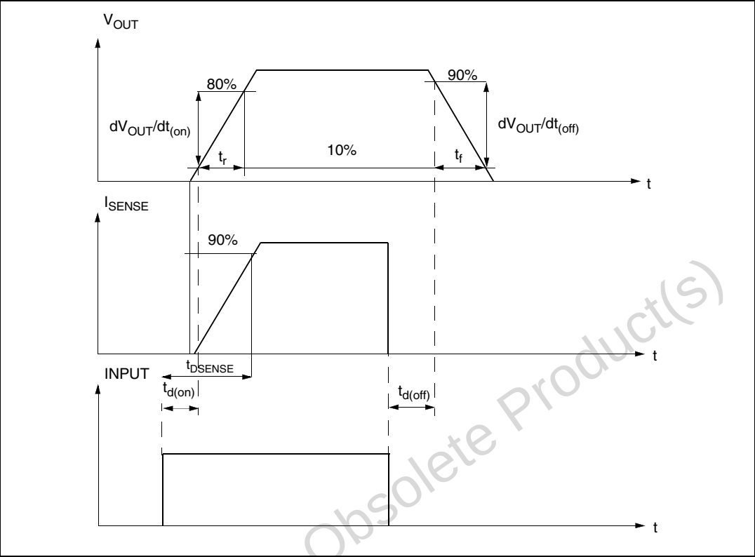
Figure 5. Switching characteristics
