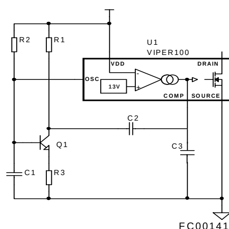
Figure 20. Slope Compensation
