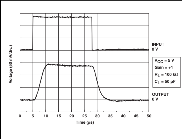
Figure 19. Slew rate vs. time for small input voltage signal
