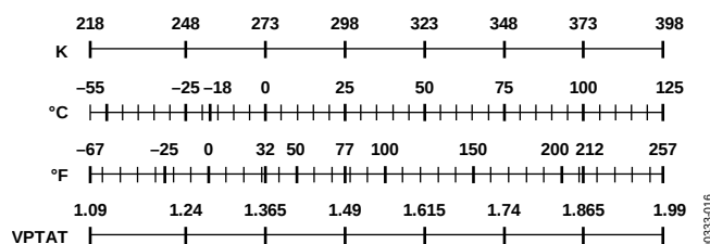
Figure 16. Temperature—VPTAT Scale
