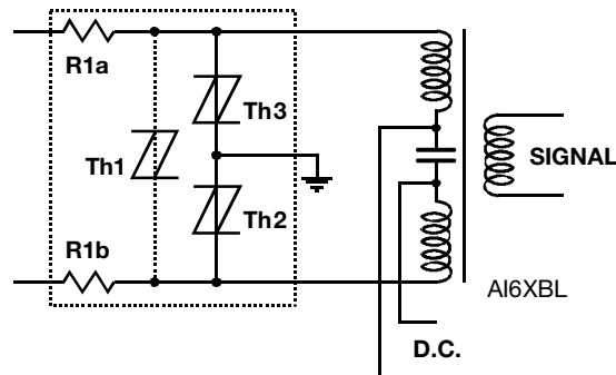
Figure 17. ISDN Protection
