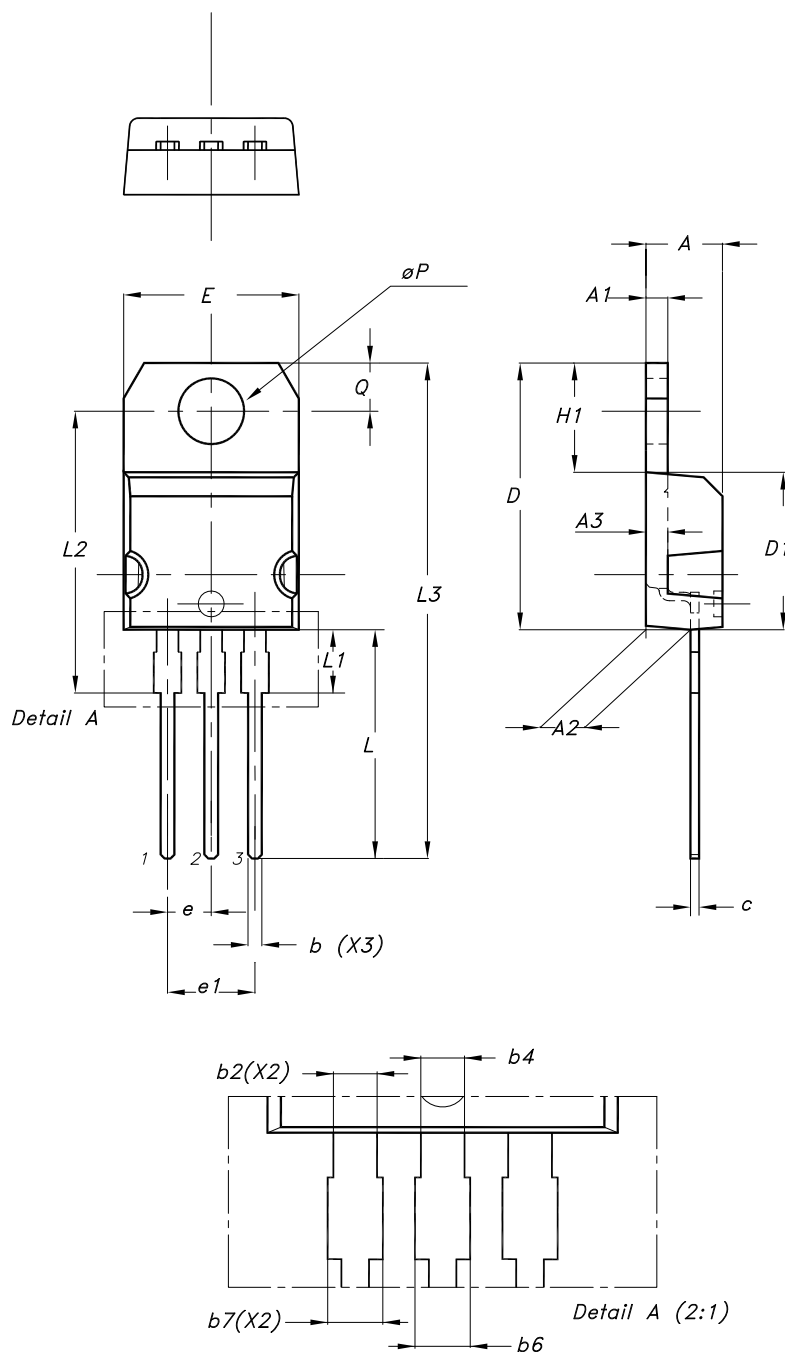
Figure 19. TO-220 type H package outline
