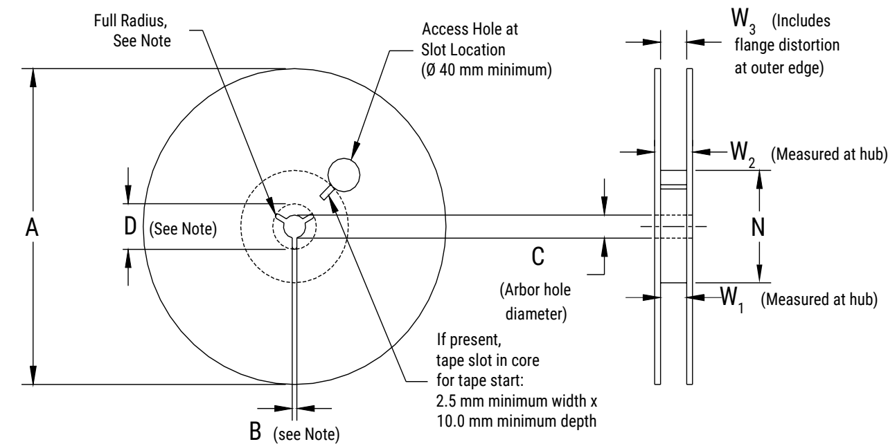
Figure 5 – Reel Dimensions
