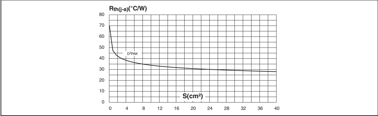
Figure 11. D 2 PAK thermal resistance junction to ambient versus copper surface under tab (printed circuit board FR4, copper thickness: 35 µm)
