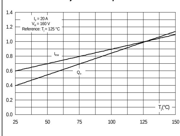
Figure 9: Relative variation of dynamic parameters versus junction temperature
