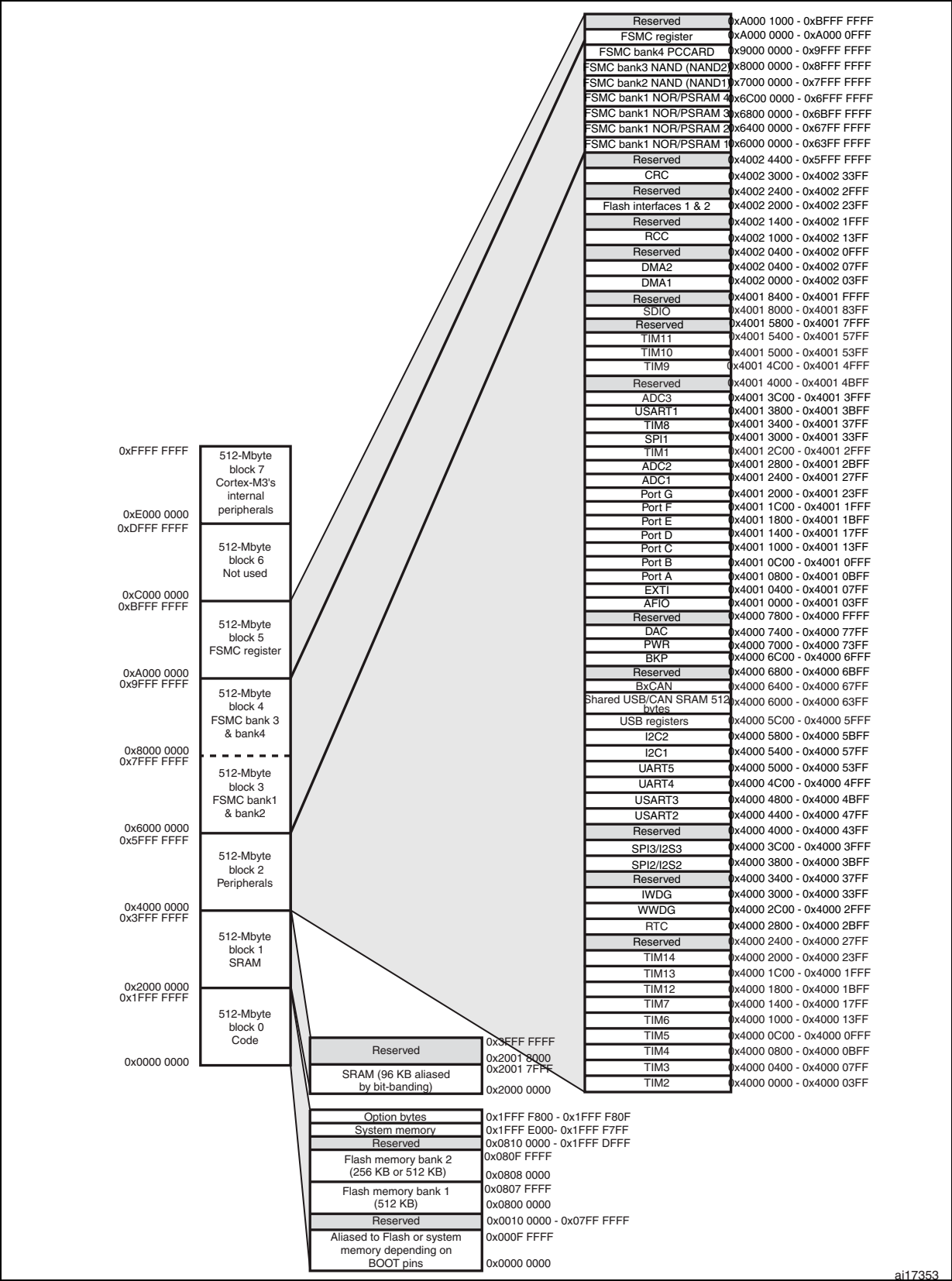
Figure 7. Memory map
