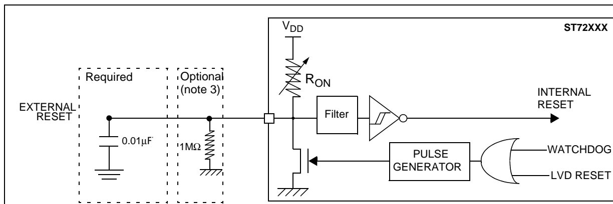
Figure 104. RESET pin protection when LVD is disabled. 1)
