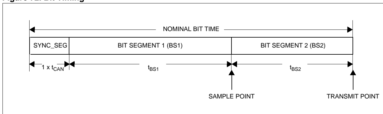
Figure 72. Bit Timing
