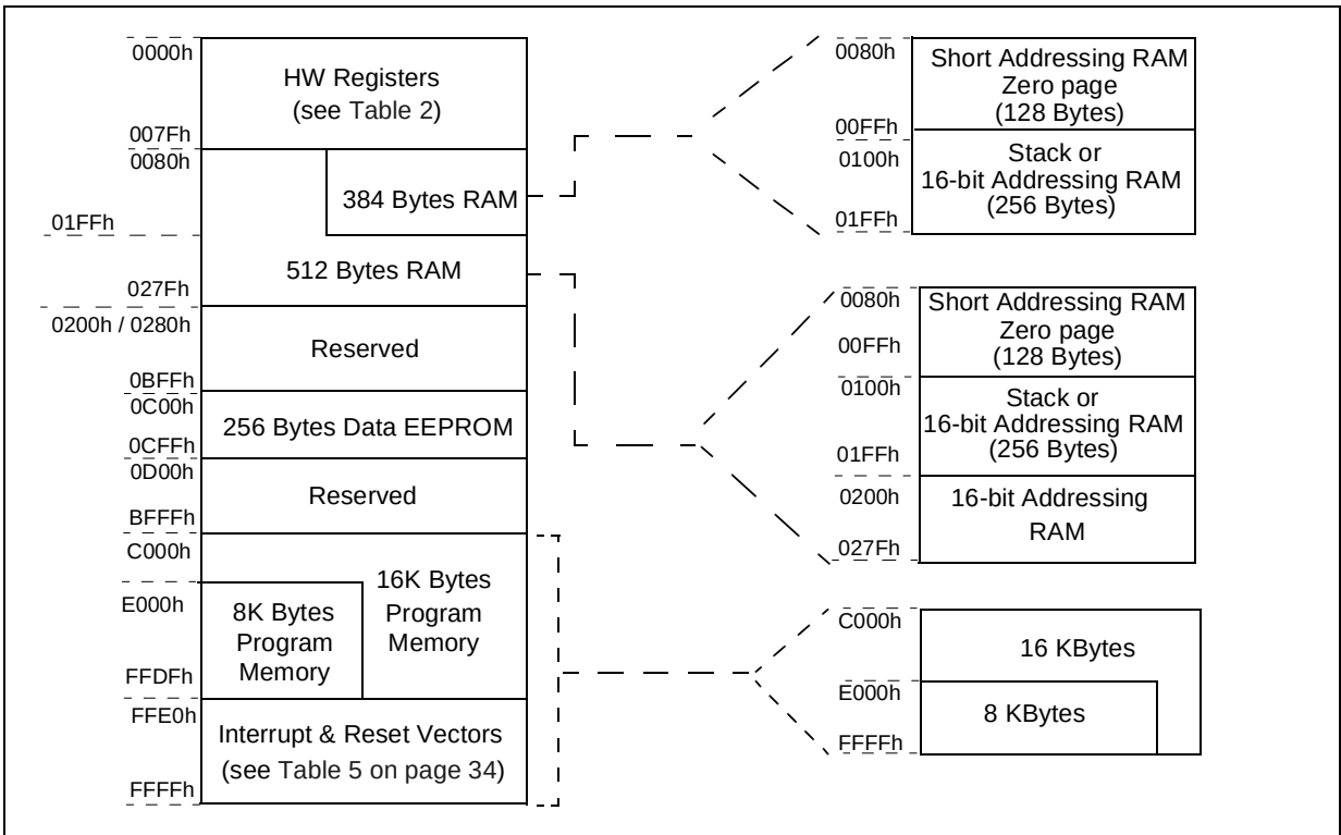
Figure 5. Memory Map
