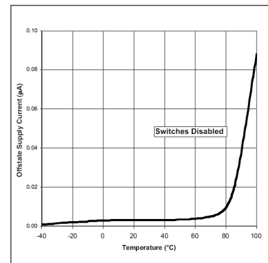
Fig. 9: Off-state Supply Current vs Temperature
