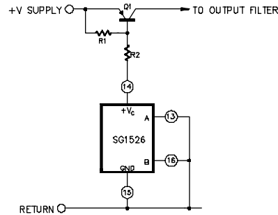
FIGURE 24. SINGLE-ENDED CONFIGURATION
