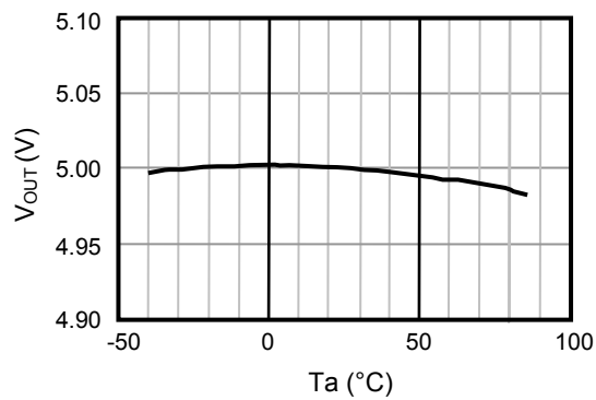
S-812C50B
