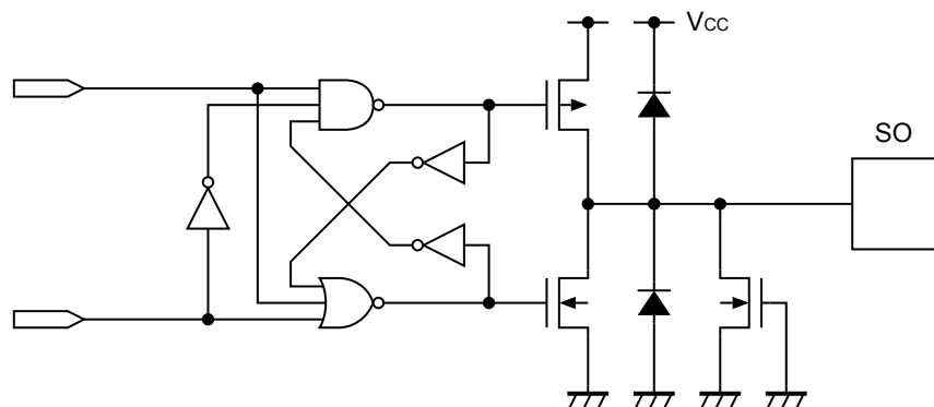
Figure 27 SO Pin
