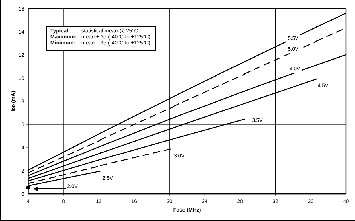
FIGURE 23-7: MAXIMUM I_{DD} vs. F_{osc} OVER V_{DD} PRI_RUN, EC MODE, -40°C TO +125°C
