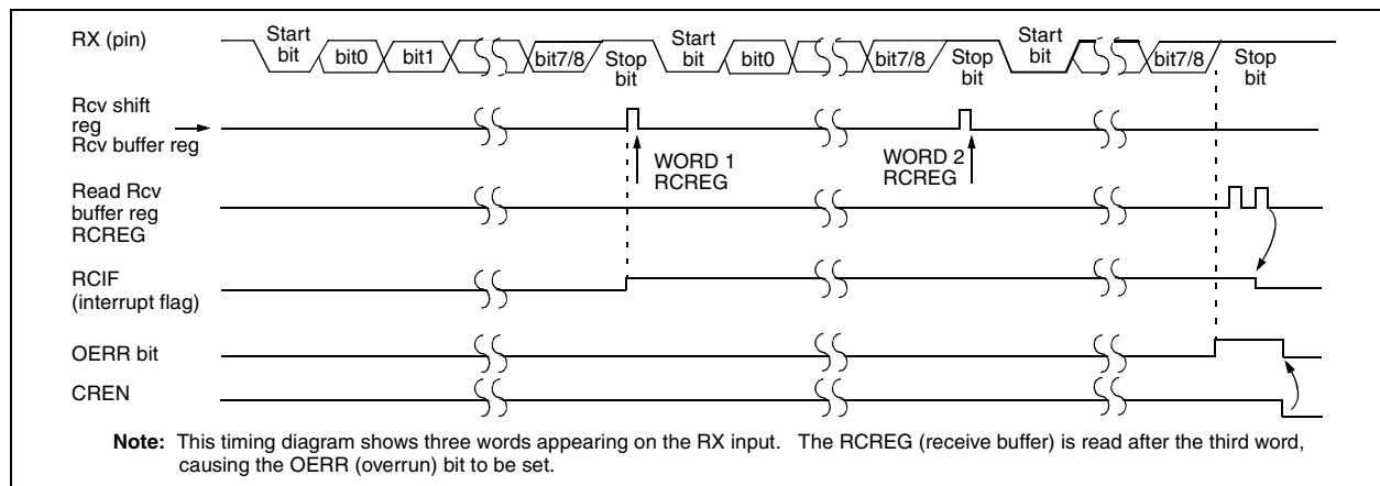
FIGURE 11-5: ASYNCHRONOUS RECEPTION
