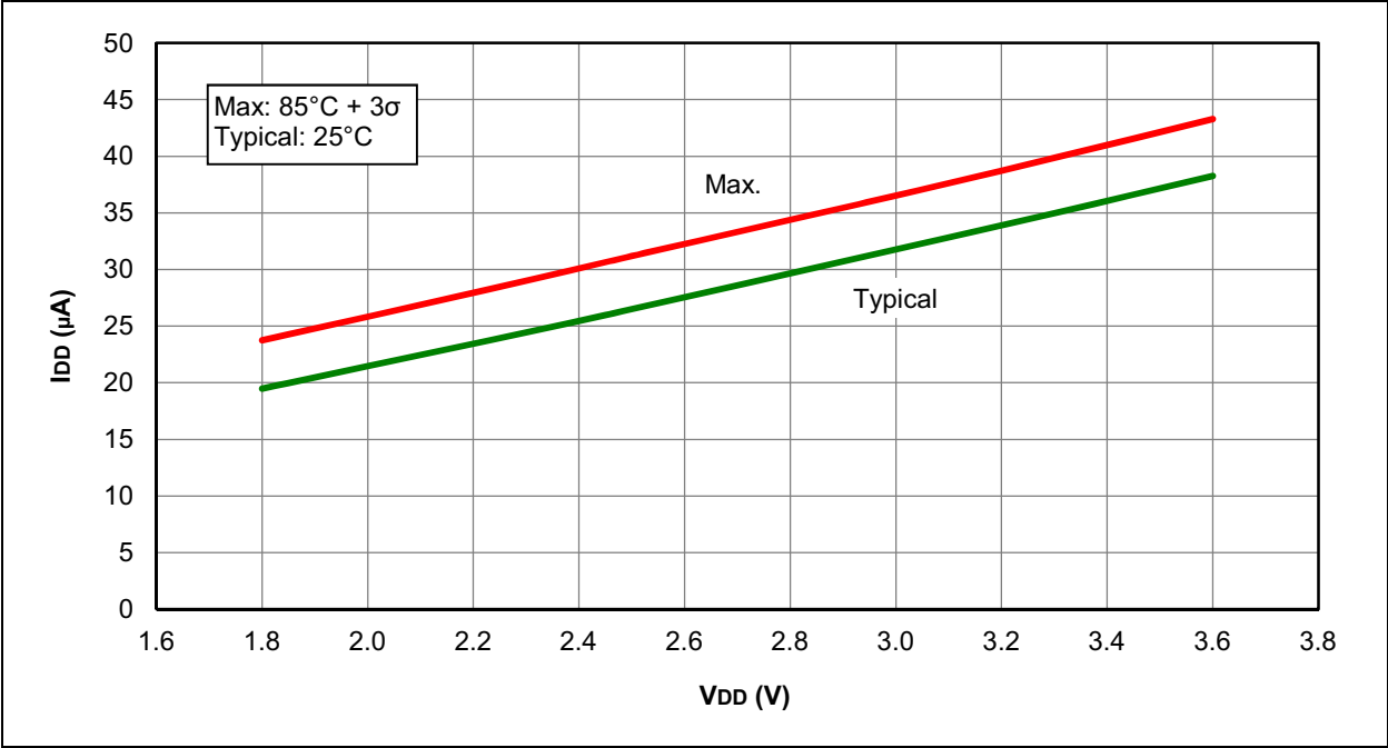
FIGURE 28-3: I_{DD} , EXTERNAL CLOCK (ECL), LOW-POWER MODE, F_{osc} = 500\text{ kHz} , PIC12LF1501 ONLY
