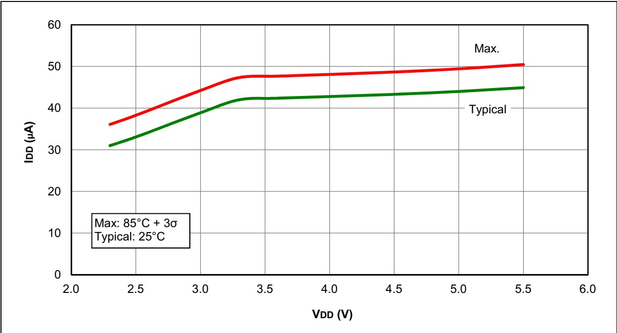
FIGURE 28-4: I_{DD} , EXTERNAL CLOCK (ECL), LOW-POWER MODE, F_{osc} = 500\text{ kHz} , PIC12F1501 ONLY
