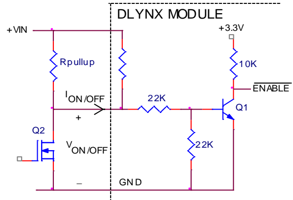
Figure 39. Circuit configuration for using positive On/Off logic.
