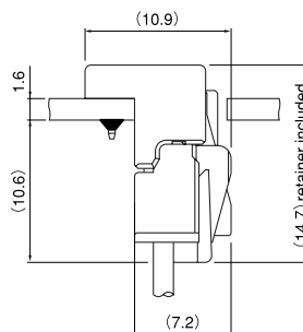
PA Receptacle (Retainer mountable type) + PA bottom type header (Extended length type)
