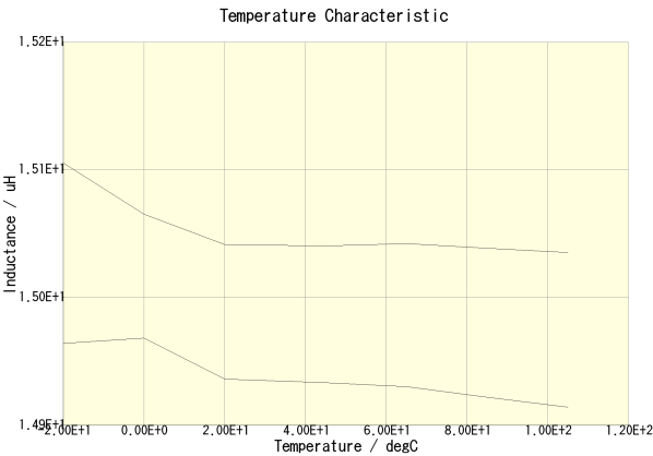
NLV25T-150J-PF(DC = 0A)
