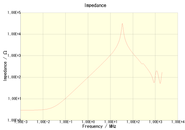
NLV25T-150J-PF
