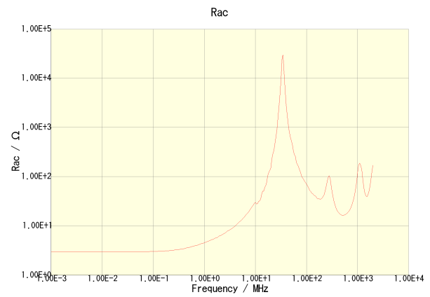
NLV25T-150J-PF
