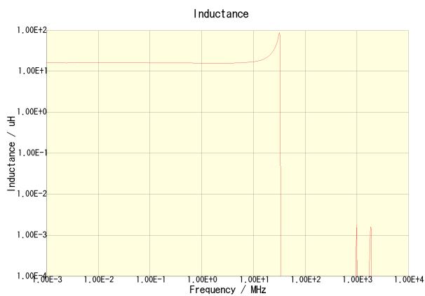
NLV25T-150J-PF
