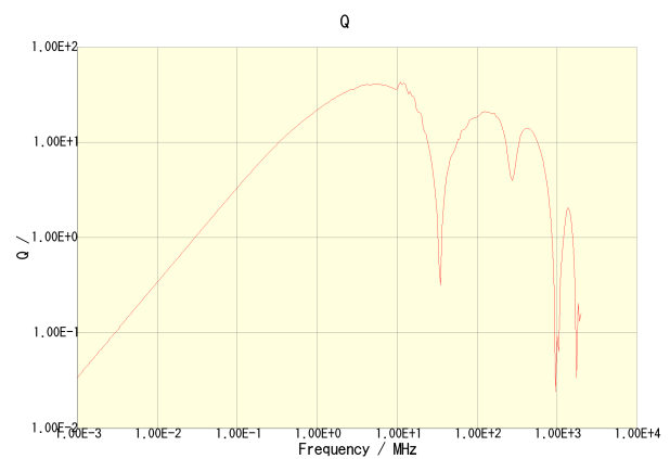
NLV25T-150J-PF
