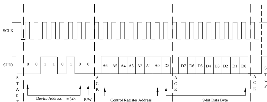
Figure 21: Byte Write Sequence
