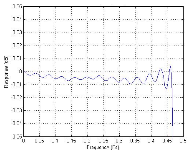
Figure 41: DAC Filter Ripple
