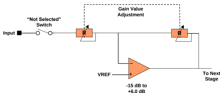
Figure 7: Variable Gain Stage Simplified Schematic
