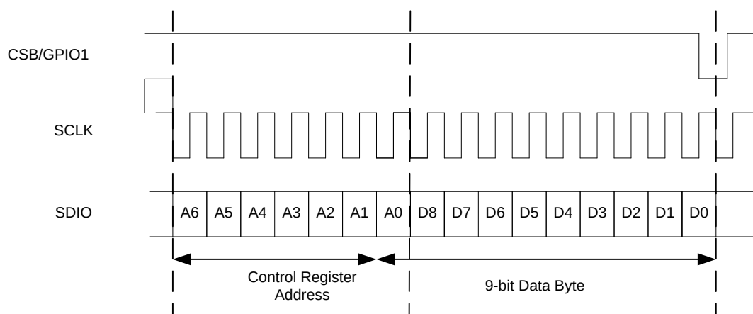
Figure 13: Register write operation using a 16-bit SPI Interface
