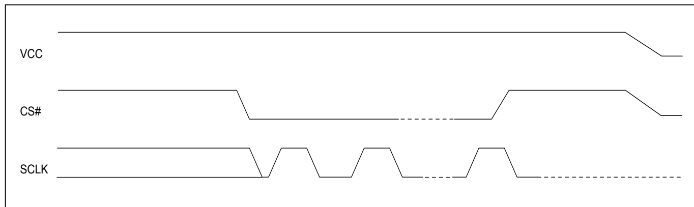
Figure 29. Power-Down Sequence
