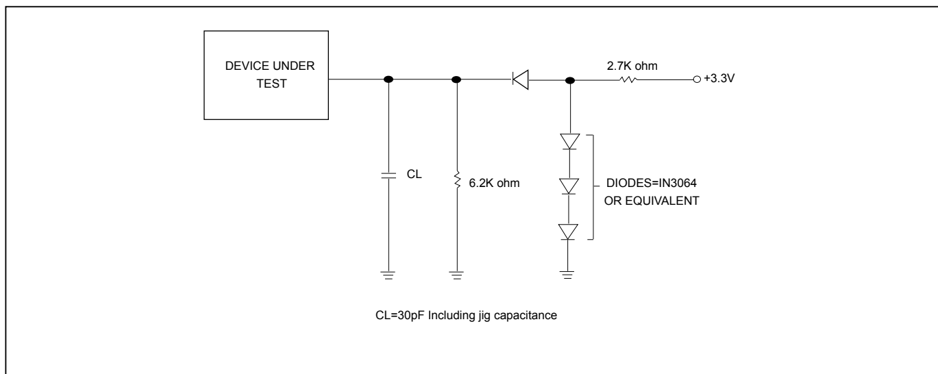
Figure 6. OUTPUT LOADING
