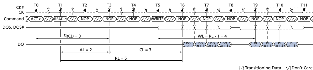
Figure 52: READ-to-WRITE
