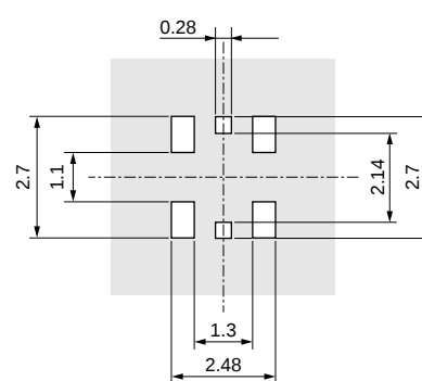
Standard Solder Stencil Mask Pattern (Mask thickness 0.12mm)
