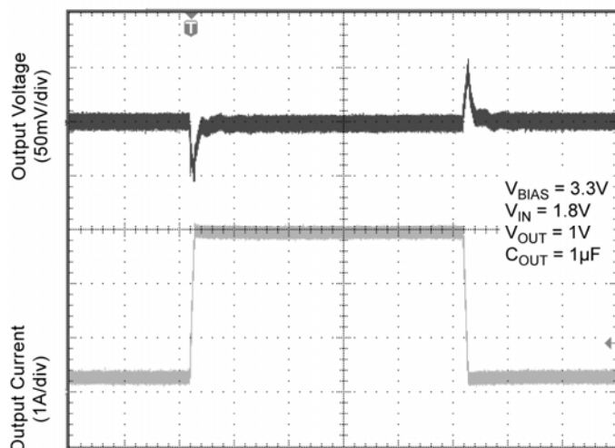
Load Transient
