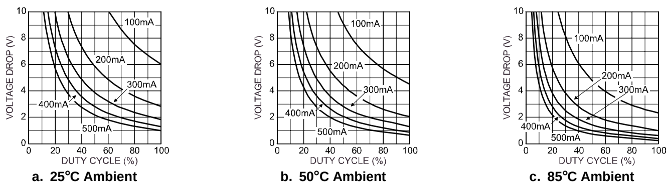
Figure 3. MIC5216-x.xBMM (MSOP-8) on Minimum Recommended Footprint
