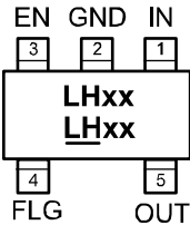
MIC5216-xxBM5/YM5 SOT-23-5 Fixed Voltages
