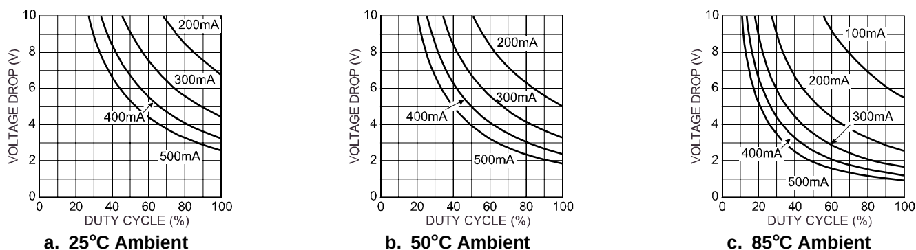
Figure 4. MIC5216-x.xBMM (MSOP-8) on 1-inch 2 Copper Cladding
