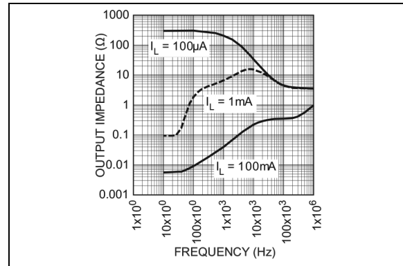
FIGURE 2-22: Output Impedance.
